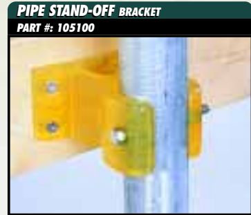
Polyurethane bracket attaches top of pipe to stationary docks. Fits pipe from 2.5" (6cm) to 3.5" (9cm) O.D.
