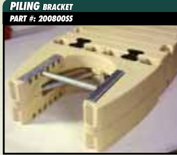
Heavy-duty polyethylene bracket allows lateral position adjustment to attach to piles up to 18" (46cm) in diameter.
